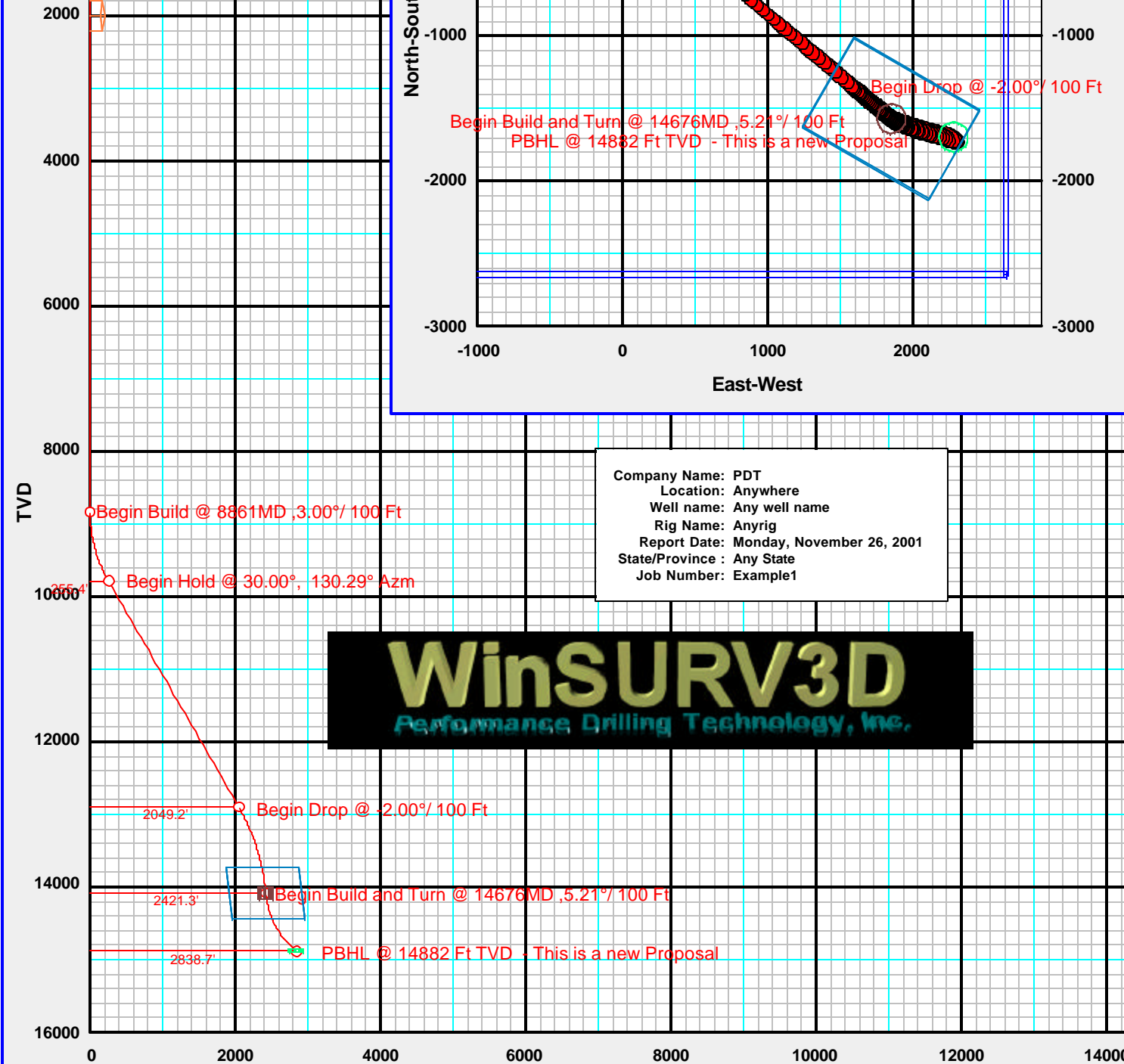
Vertical Section @ 126.65°
